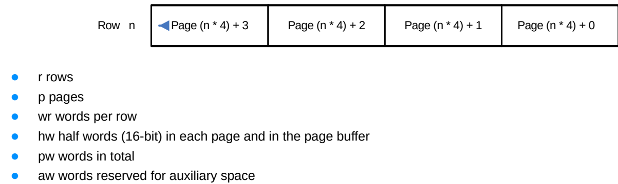
Figure 20-2. Row Organization
