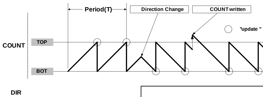
Figure 27-3. Counter Operation
