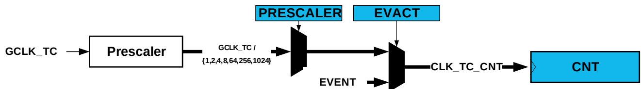
Figure 27-2. Prescaler
