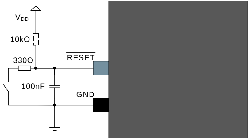
Figure 34-4. External Reset Circuit Example Schematic
