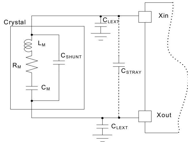
Figure 32-4. Oscillator Connection
