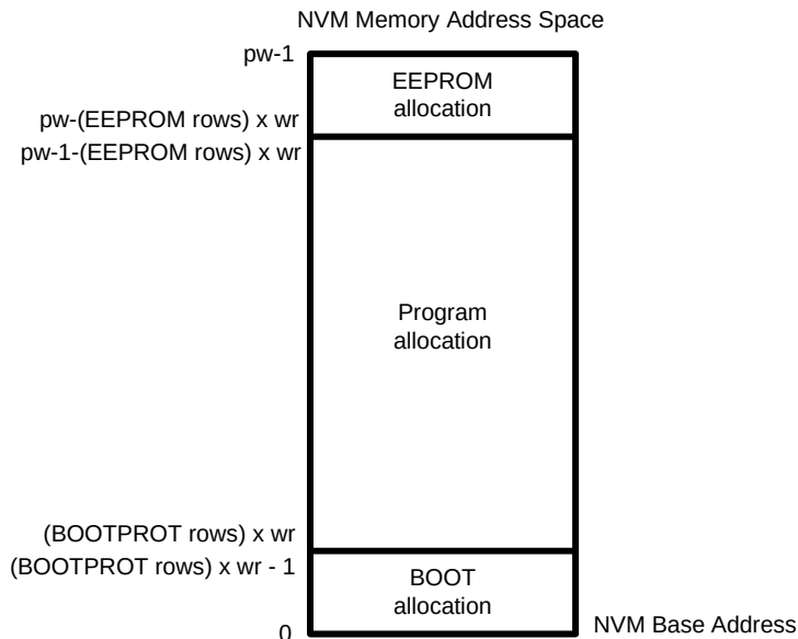
Figure 20-4. EEPROM and BOOT Allocation
