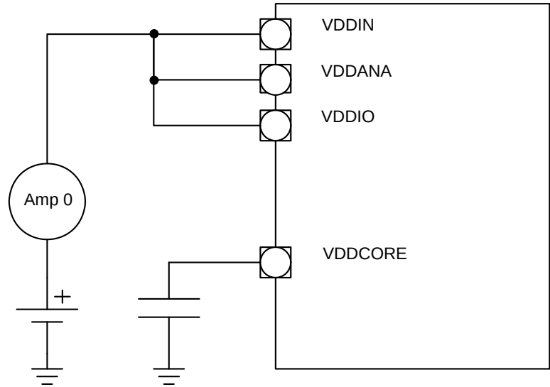
Figure 32-1. Measurements Schematics
