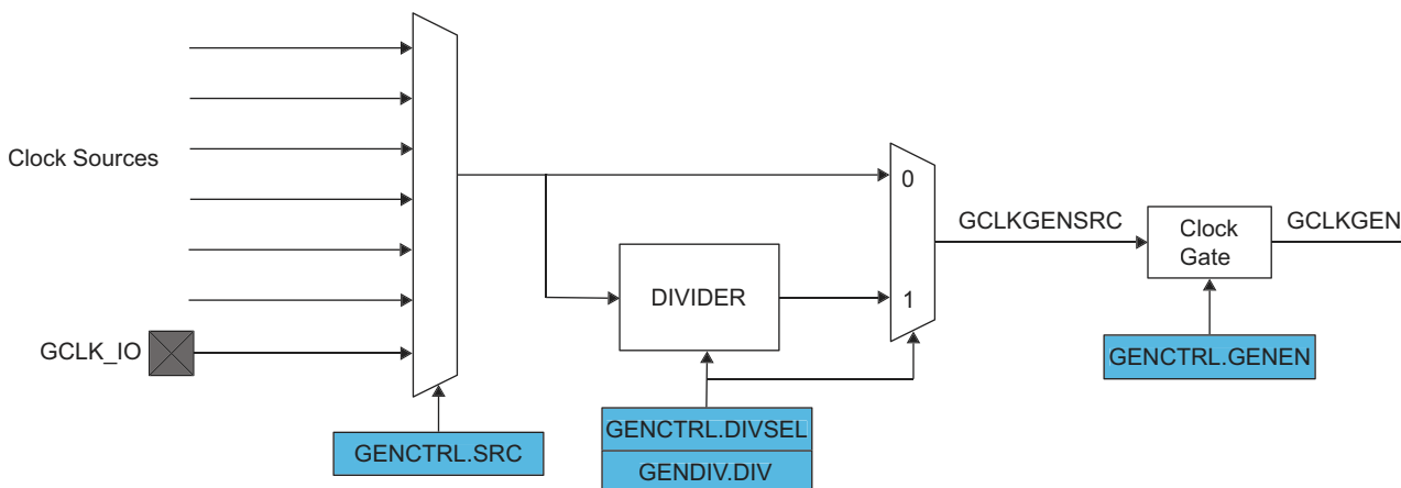
Figure 14-3. Generic Clock Generator
